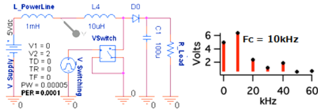
Figure 1: (Left) Circuit model of a SMPS with placement of the voltage probe. (Right) Frequency domain analysis at the voltage probe from probe showing EMI at 10 kHz.
